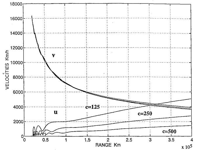
Fig. 5 Spacecraft velocity components vs range to central body for various positive values of guidance parameter c .
